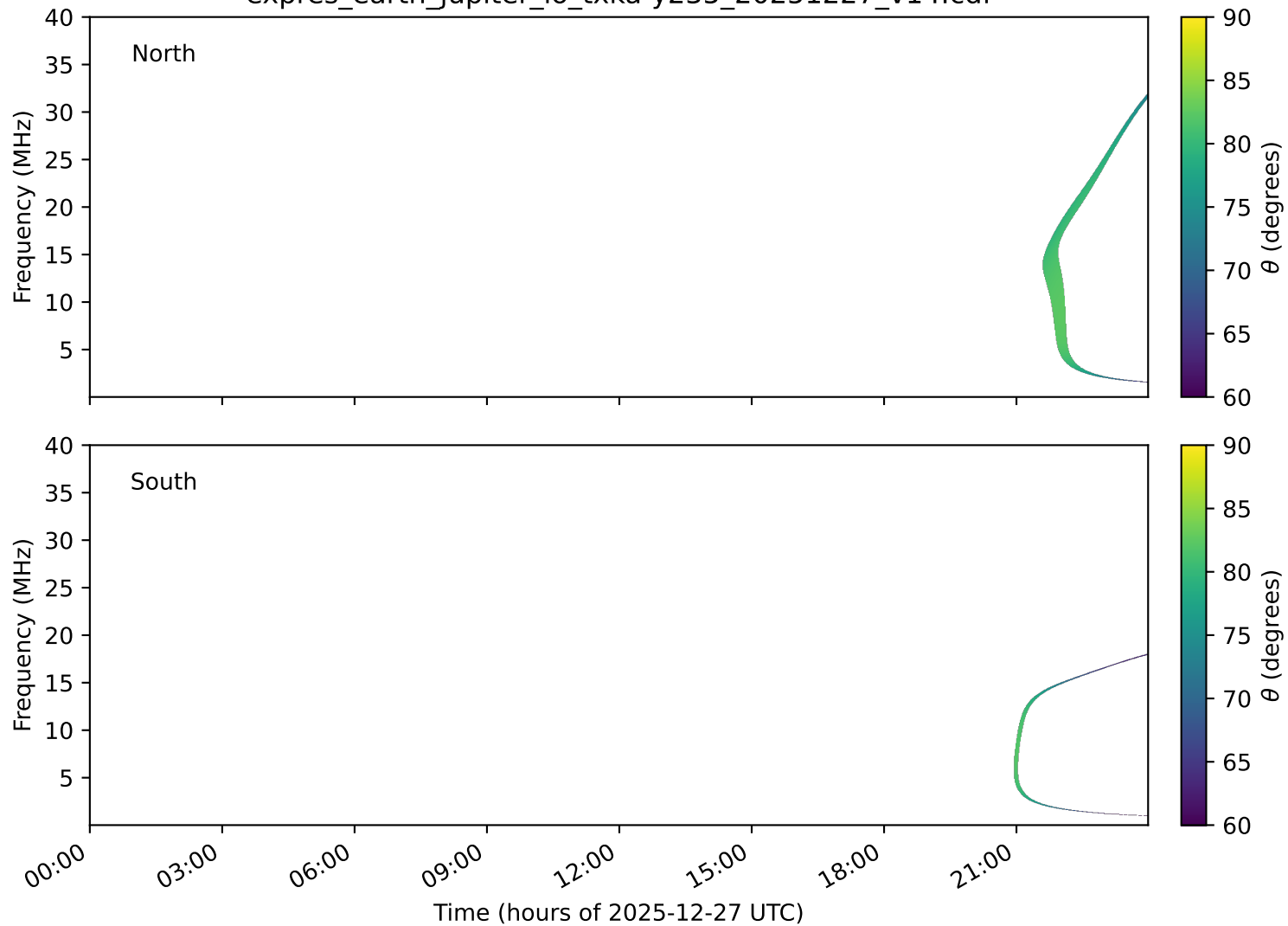
expres_earth_jupiter_io_txka-y235_20251227_v14.cdf
