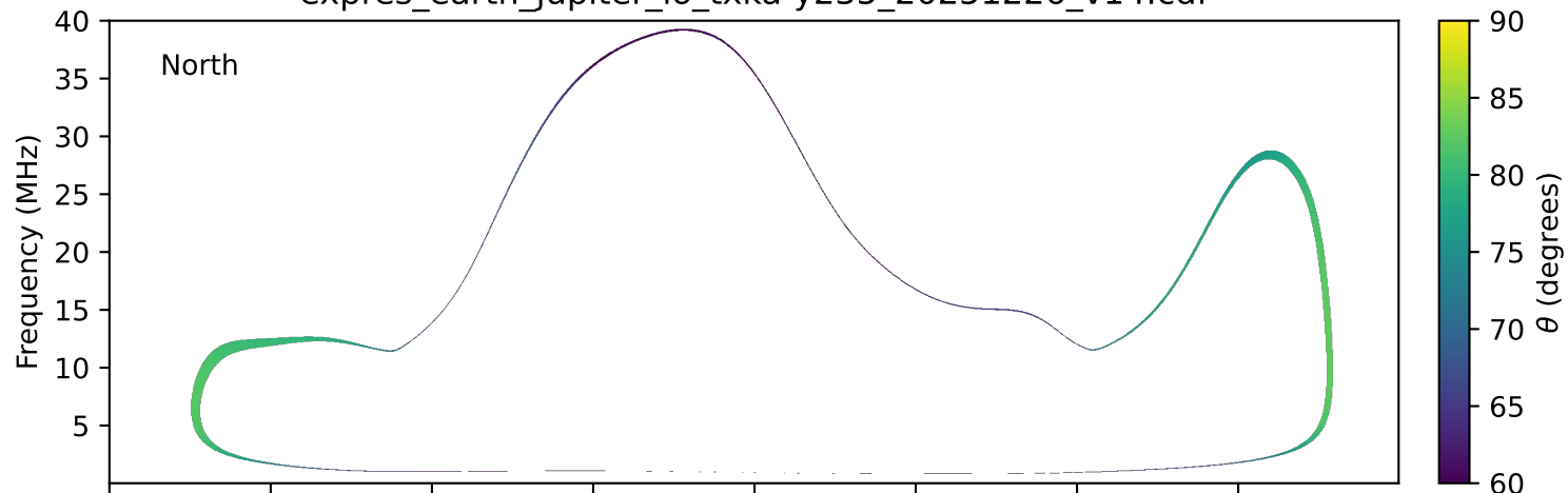
expres_earth_jupiter_io_txka-y235_20251226_v14.cdf
