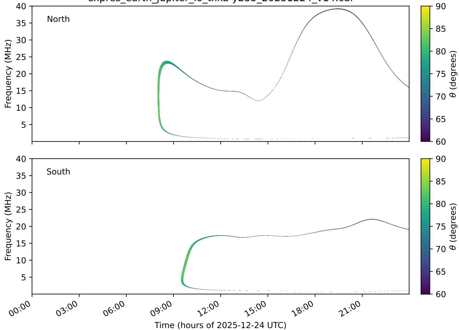
expres_earth_jupiter_io_txka-y235_20251224_v14.cdf
