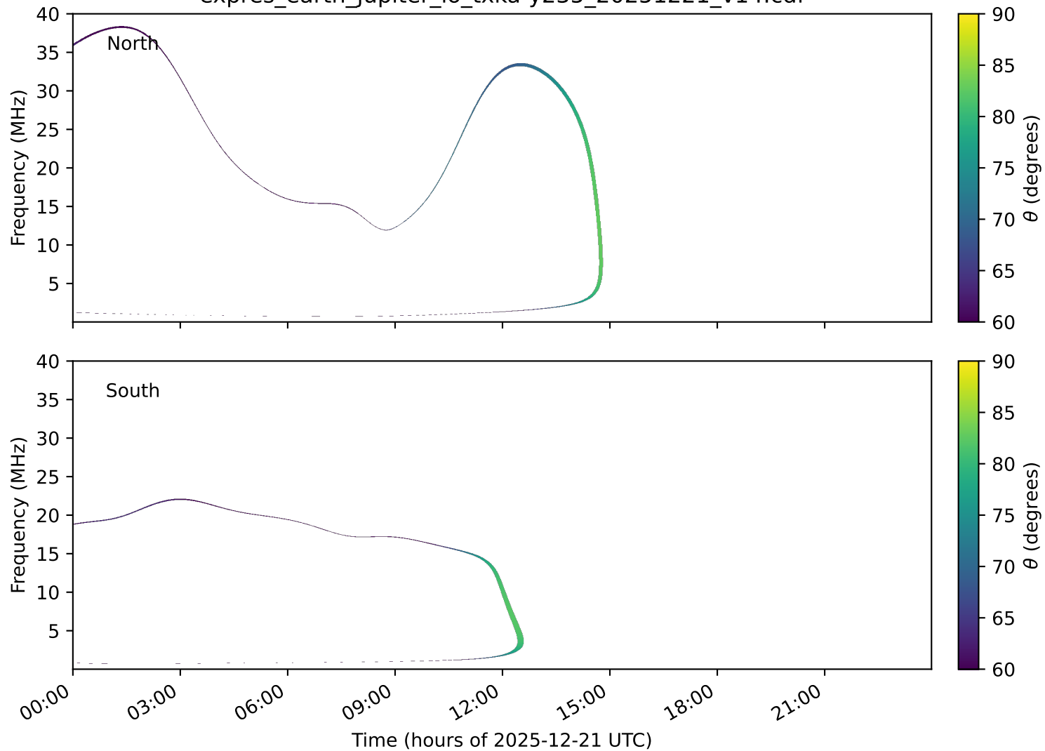
expres_earth_jupiter_io_txka-y235_20251221_v14.cdf
