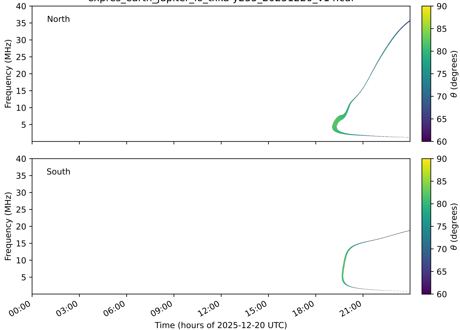
expres_earth_jupiter_io_txka-y235_20251220_v14.cdf
