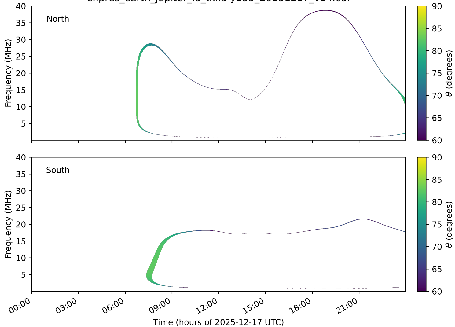
expres_earth_jupiter_io_txka-y235_20251217_v14.cdf
