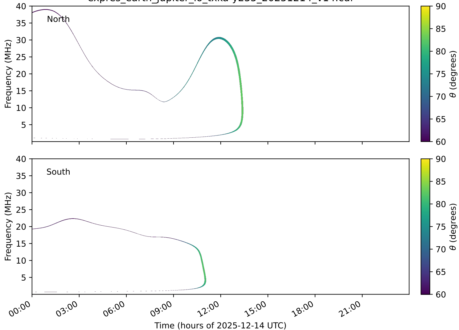
expres_earth_jupiter_io_txka-y235_20251214_v14.cdf
