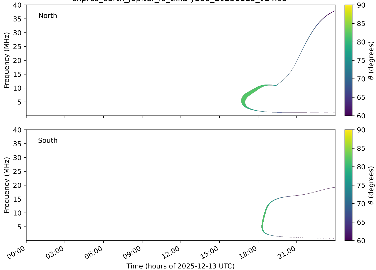
expres_earth_jupiter_io_txka-y235_20251213_v14.cdf
