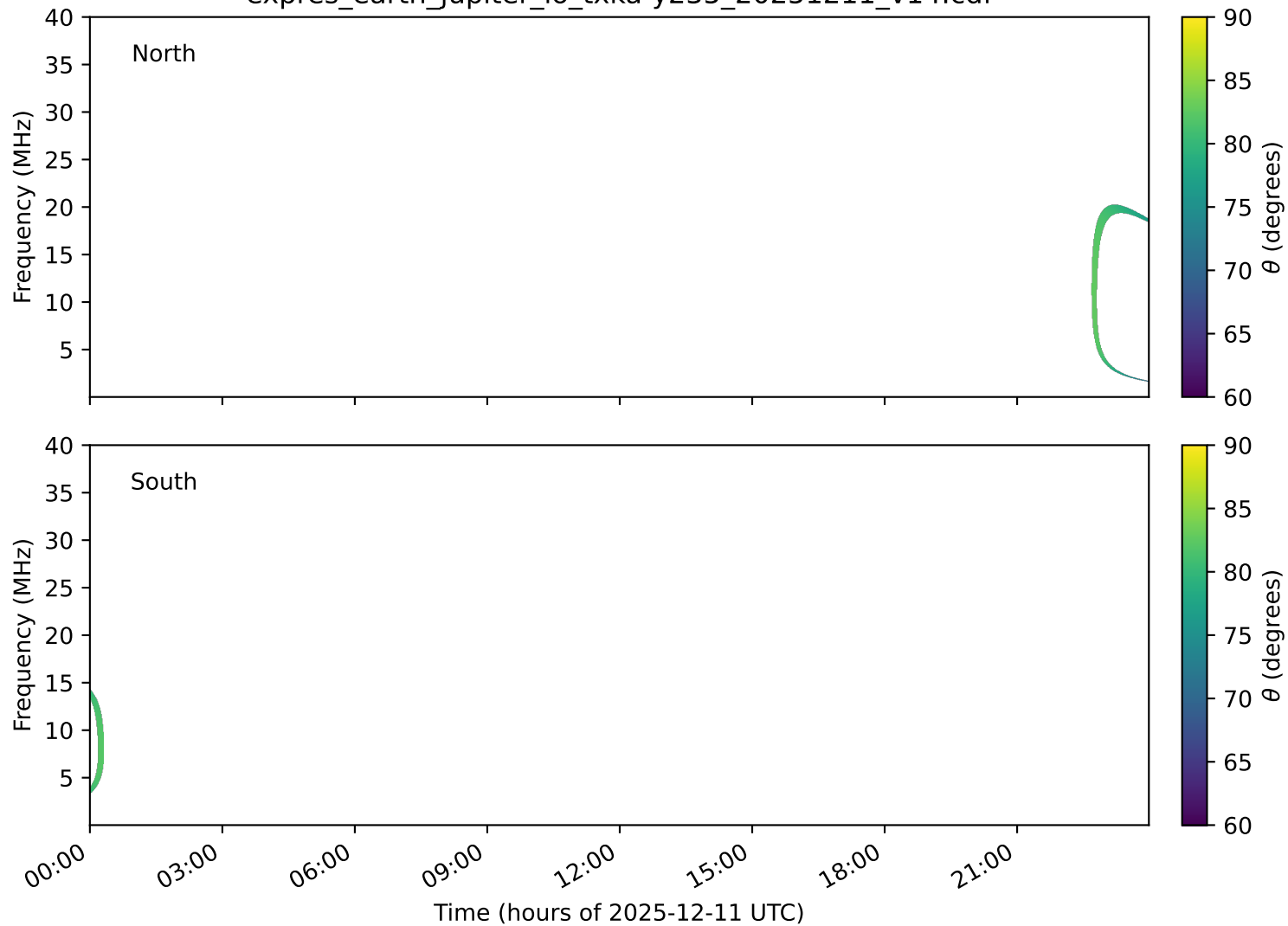
expres_earth_jupiter_io_txka-y235_20251211_v14.cdf
