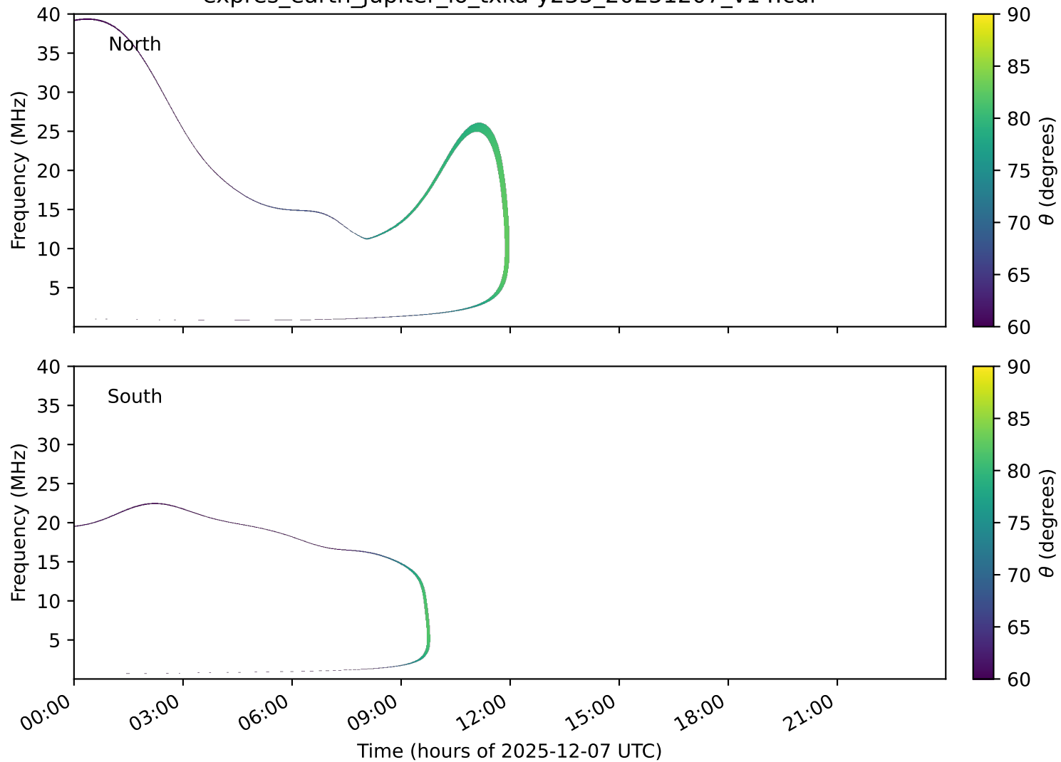
expres_earth_jupiter_io_txka-y235_20251207_v14.cdf
