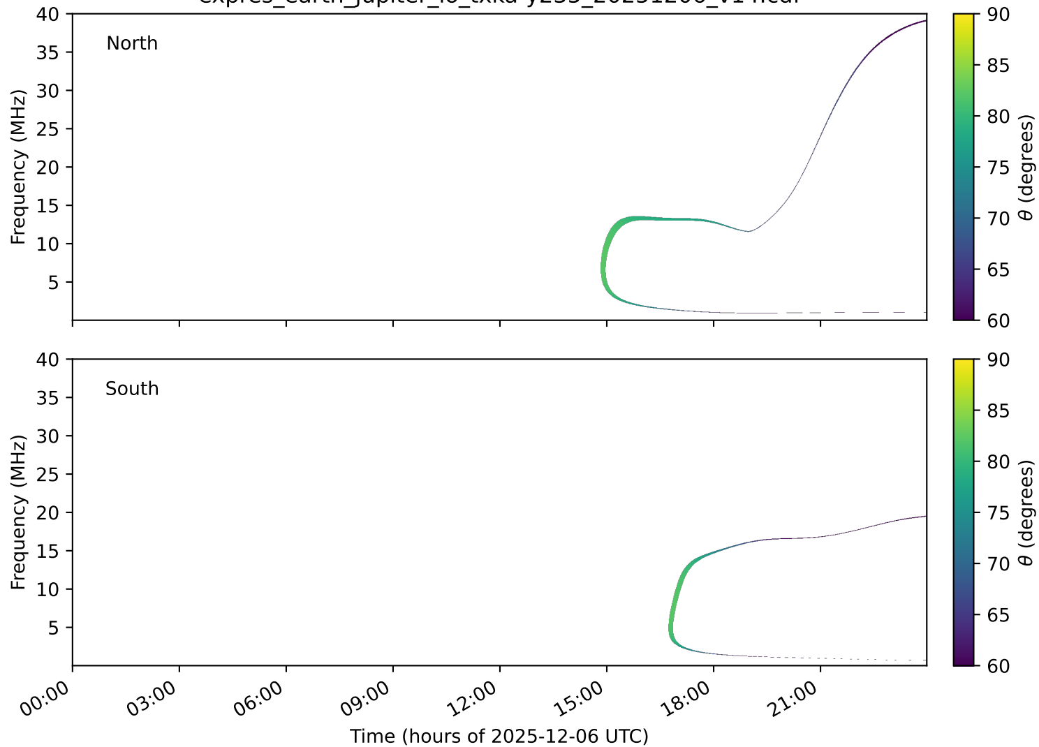
expres_earth_jupiter_io_txka-y235_20251206_v14.cdf
