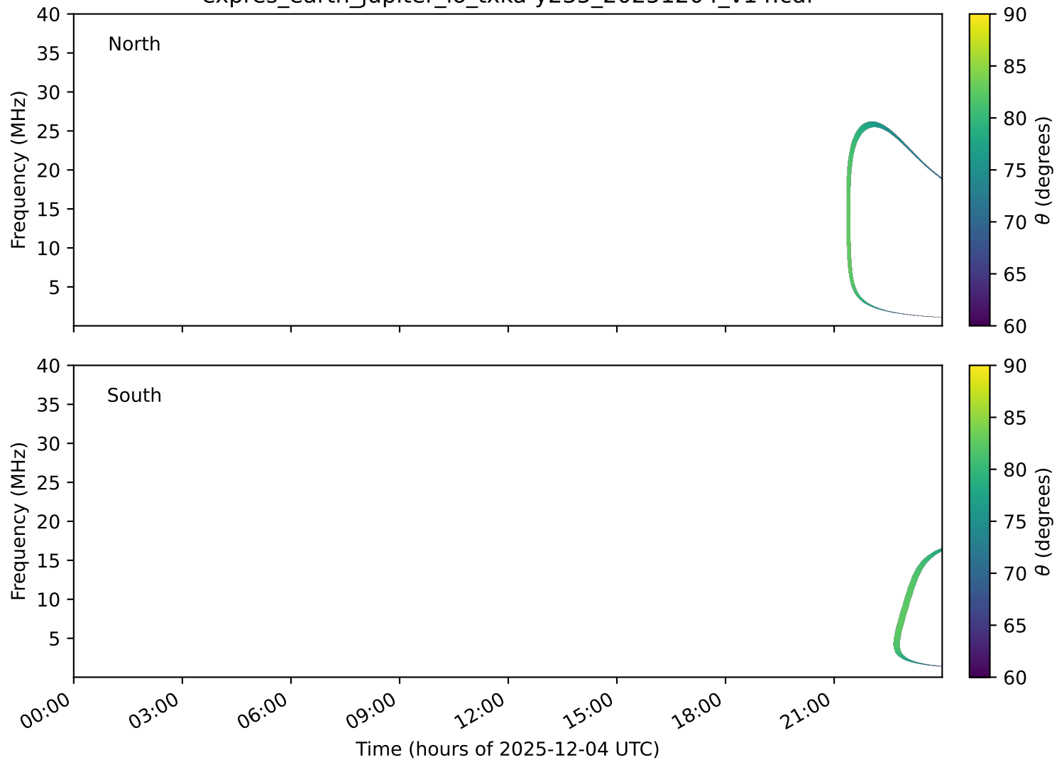
expres_earth_jupiter_io_txka-y235_20251204_v14.cdf
