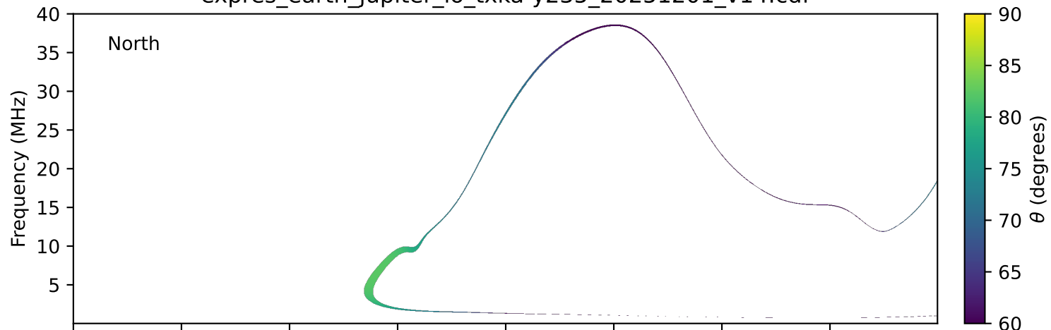
expres_earth_jupiter_io_txka-y235_20251201_v14.cdf
