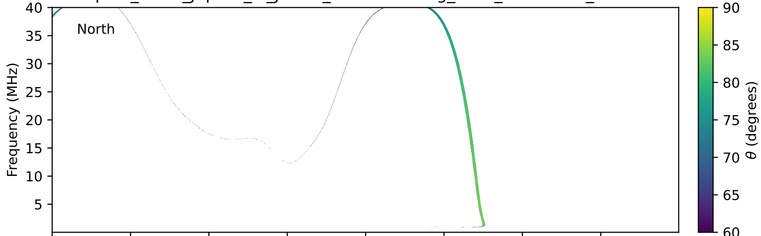
expres_earth_jupiter_io_jrm33_lossc-wid1deg_3kev_20251228_v11.cdf
