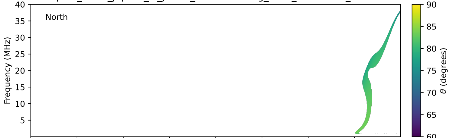
expres_earth_jupiter_io_jrm33_lossc-wid1deg_3kev_20251227_v11.cdf
