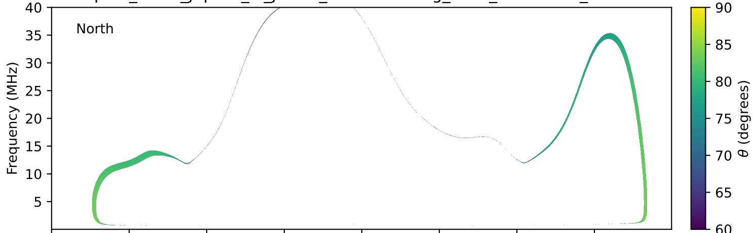
expres_earth_jupiter_io_jrm33_lossc-wid1deg_3kev_20251226_v11.cdf
