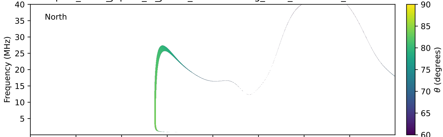
expres_earth_jupiter_io_jrm33_lossc-wid1deg_3kev_20251224_v11.cdf
