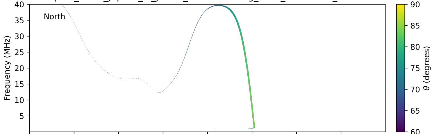
expres_earth_jupiter_io_jrm33_lossc-wid1deg_3kev_20251221_v11.cdf
