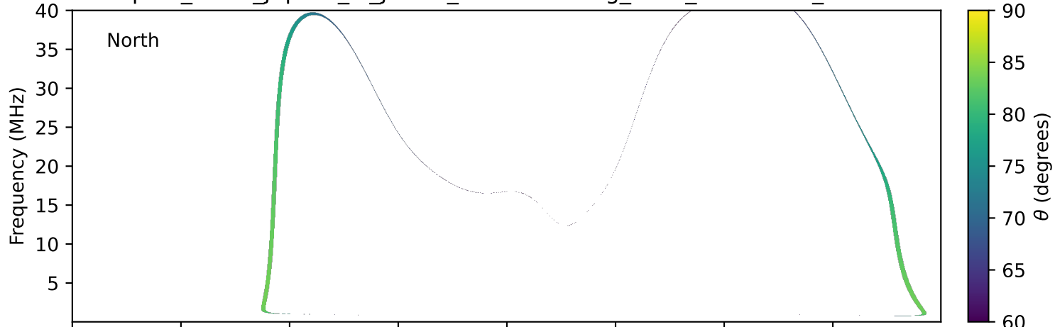
expres_earth_jupiter_io_jrm33_lossc-wid1deg_3kev_20251210_v11.cdf
