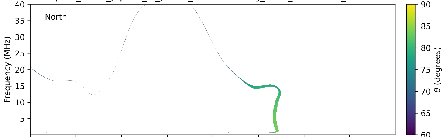
expres_earth_jupiter_io_jrm33_lossc-wid1deg_3kev_20251205_v11.cdf
