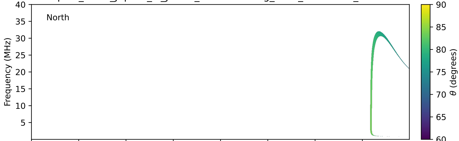
expres_earth_jupiter_io_jrm33_lossc-wid1deg_3kev_20251204_v11.cdf
