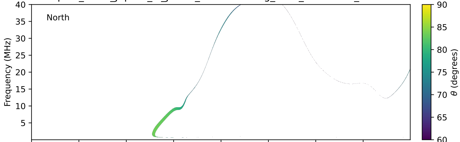
expres_earth_jupiter_io_jrm33_lossc-wid1deg_3kev_20251201_v11.cdf
