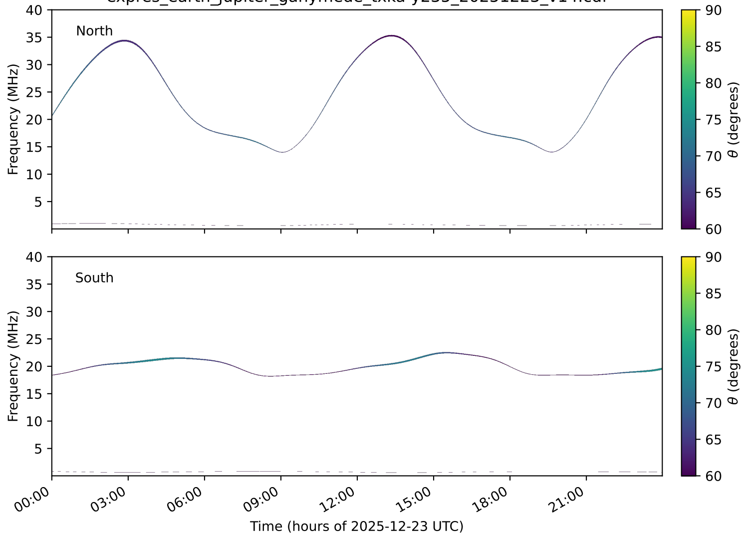
expres_earth_jupiter_ganymede_txka-y235_20251223_v14.cdf
