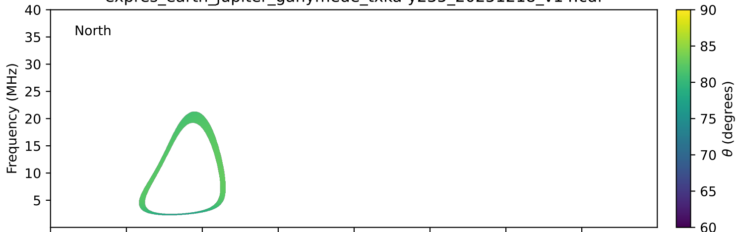
expres_earth_jupiter_ganymede_txka-y235_20251218_v14.cdf
