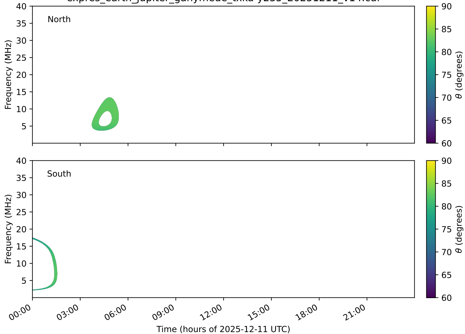
expres_earth_jupiter_ganymede_txka-y235_20251211_v14.cdf
