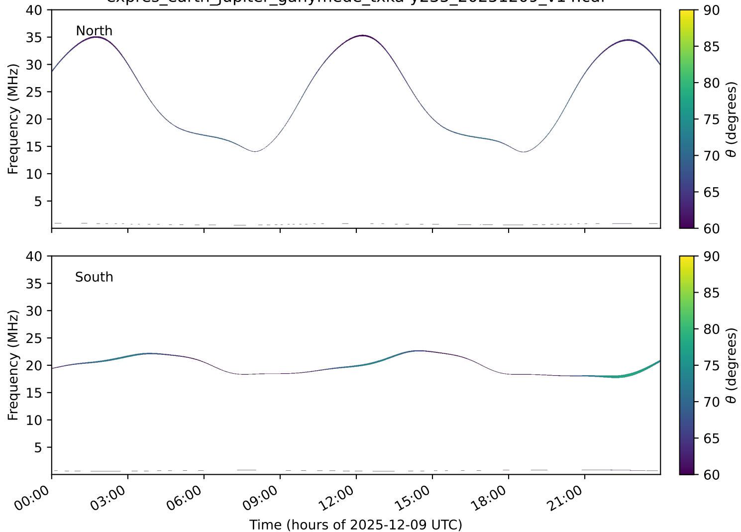
expres_earth_jupiter_ganymede_txka-y235_20251209_v14.cdf
