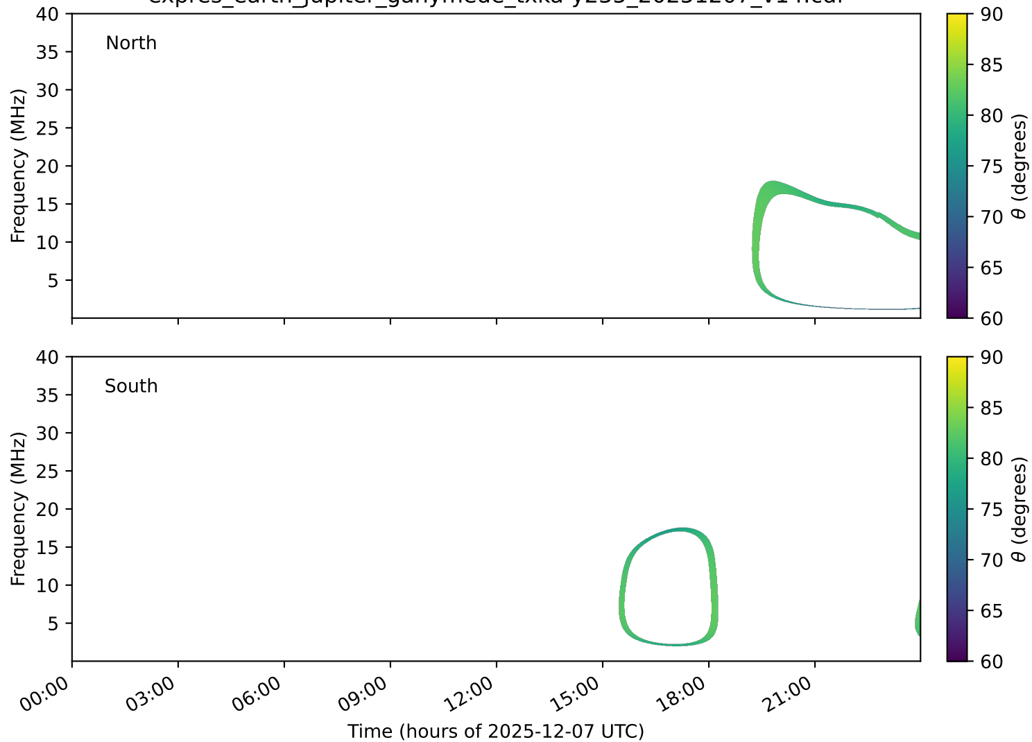
expres_earth_jupiter_ganymede_txka-y235_20251207_v14.cdf
