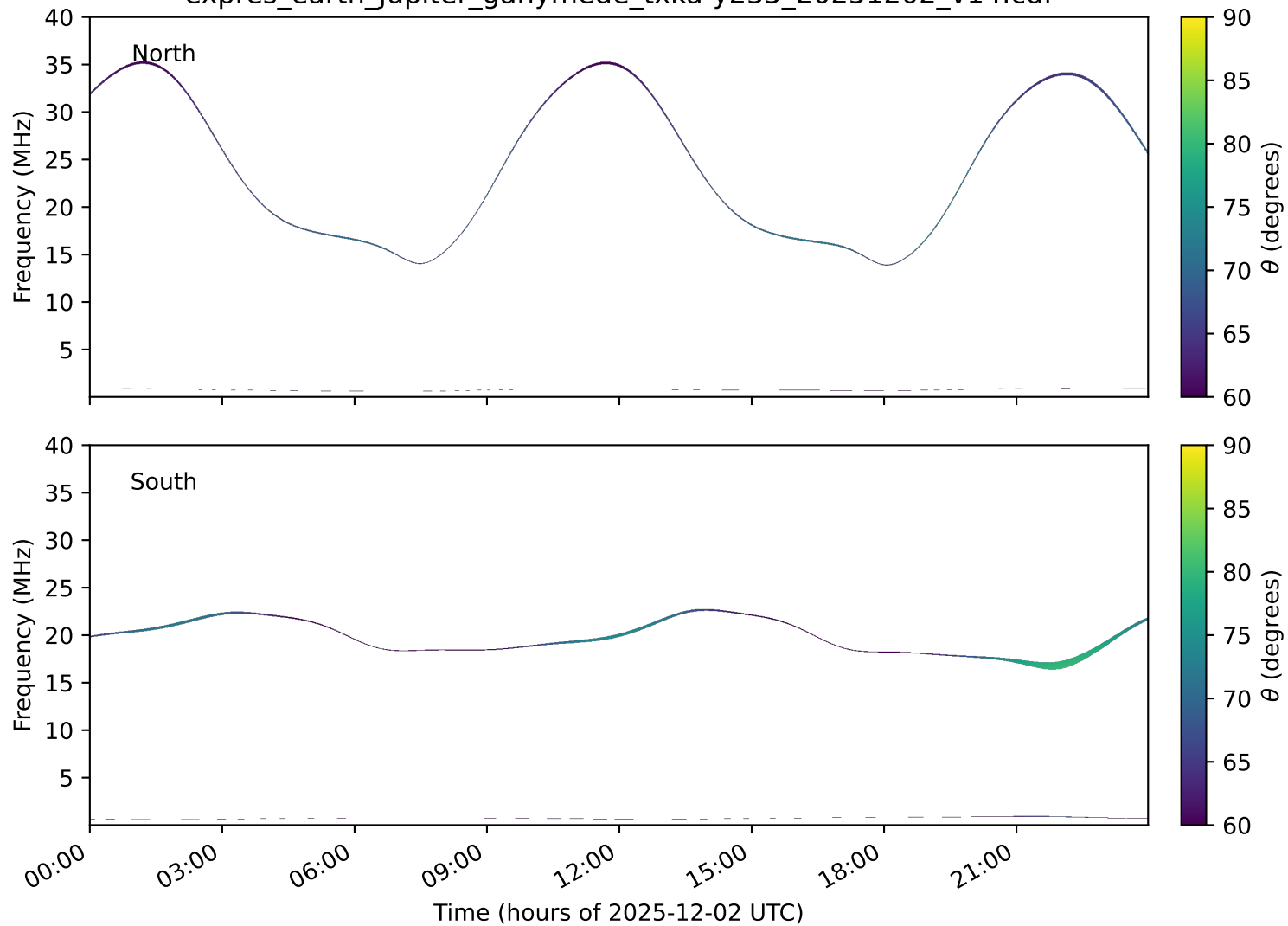
expres_earth_jupiter_ganymede_txka-y235_20251202_v14.cdf
