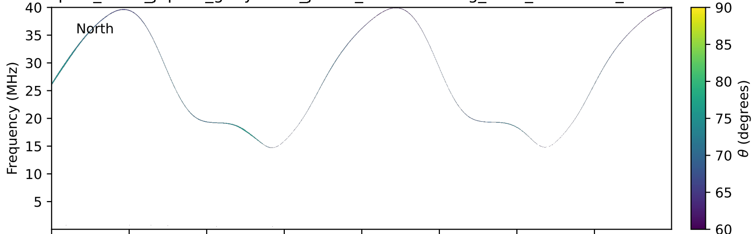
expres_earth_jupiter_ganymede_jrm33_lossc-wid1deg_3kev_20251223_v11.cdf
