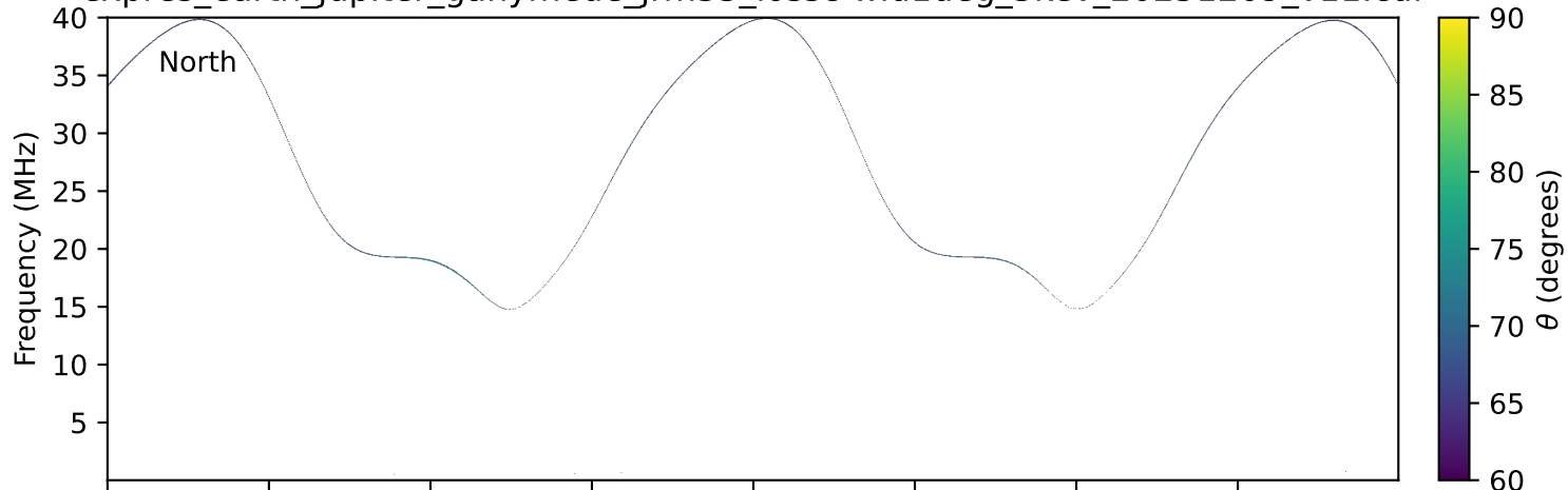
expres_earth_jupiter_ganymede_jrm33_lossc-wid1deg_3kev_20251209_v11.cdf
