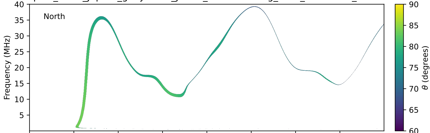
expres_earth_jupiter_ganymede_jrm33_lossc-wid1deg_3kev_20251208_v11.cdf
