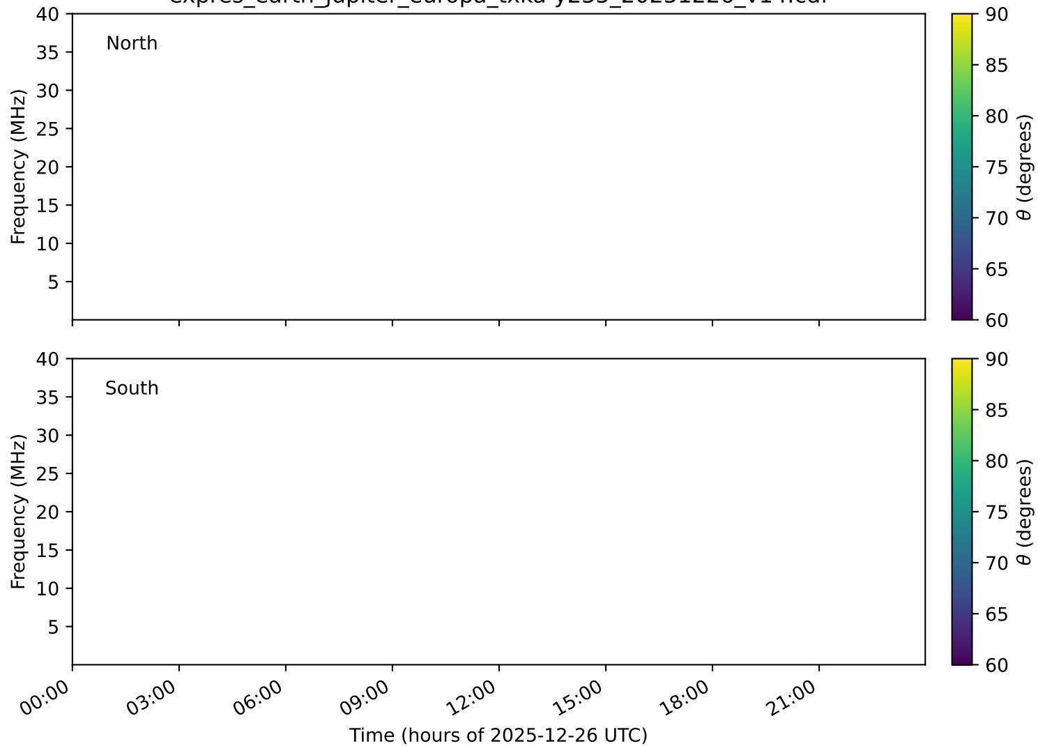
expres_earth_jupiter_europa_txka-y235_20251226_v14.cdf
