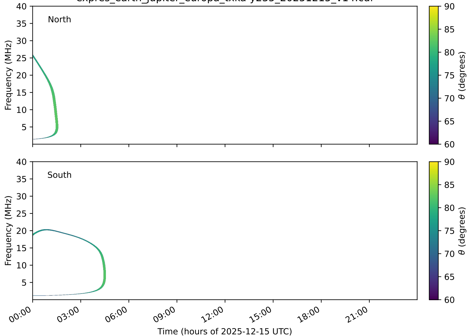
expres_earth_jupiter_europa_txka-y235_20251215_v14.cdf
