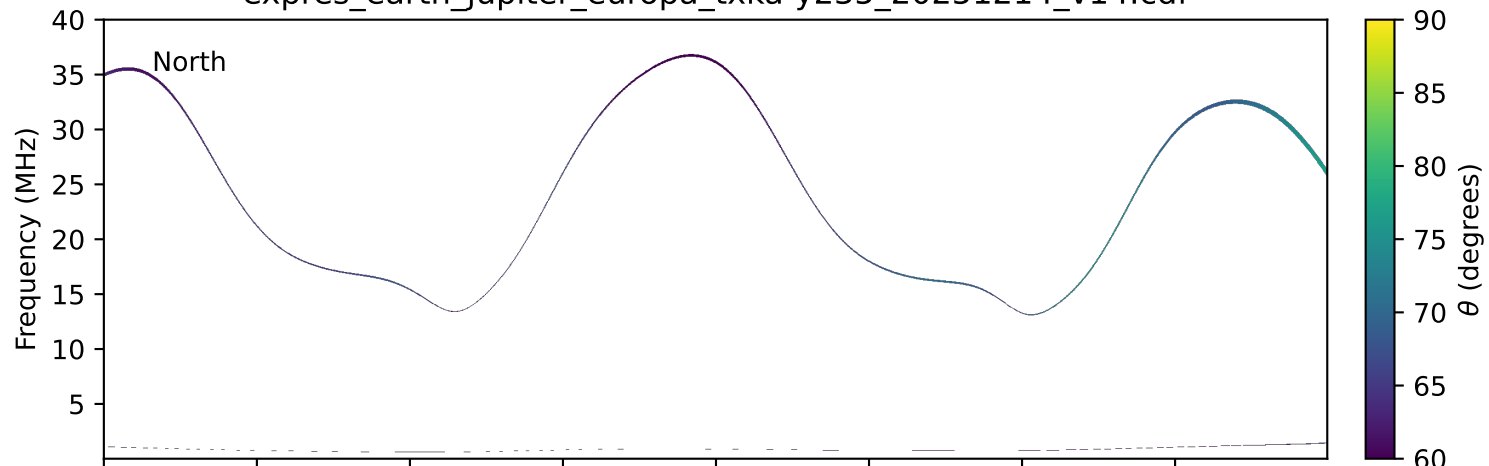
expres_earth_jupiter_europa_txka-y235_20251214_v14.cdf
