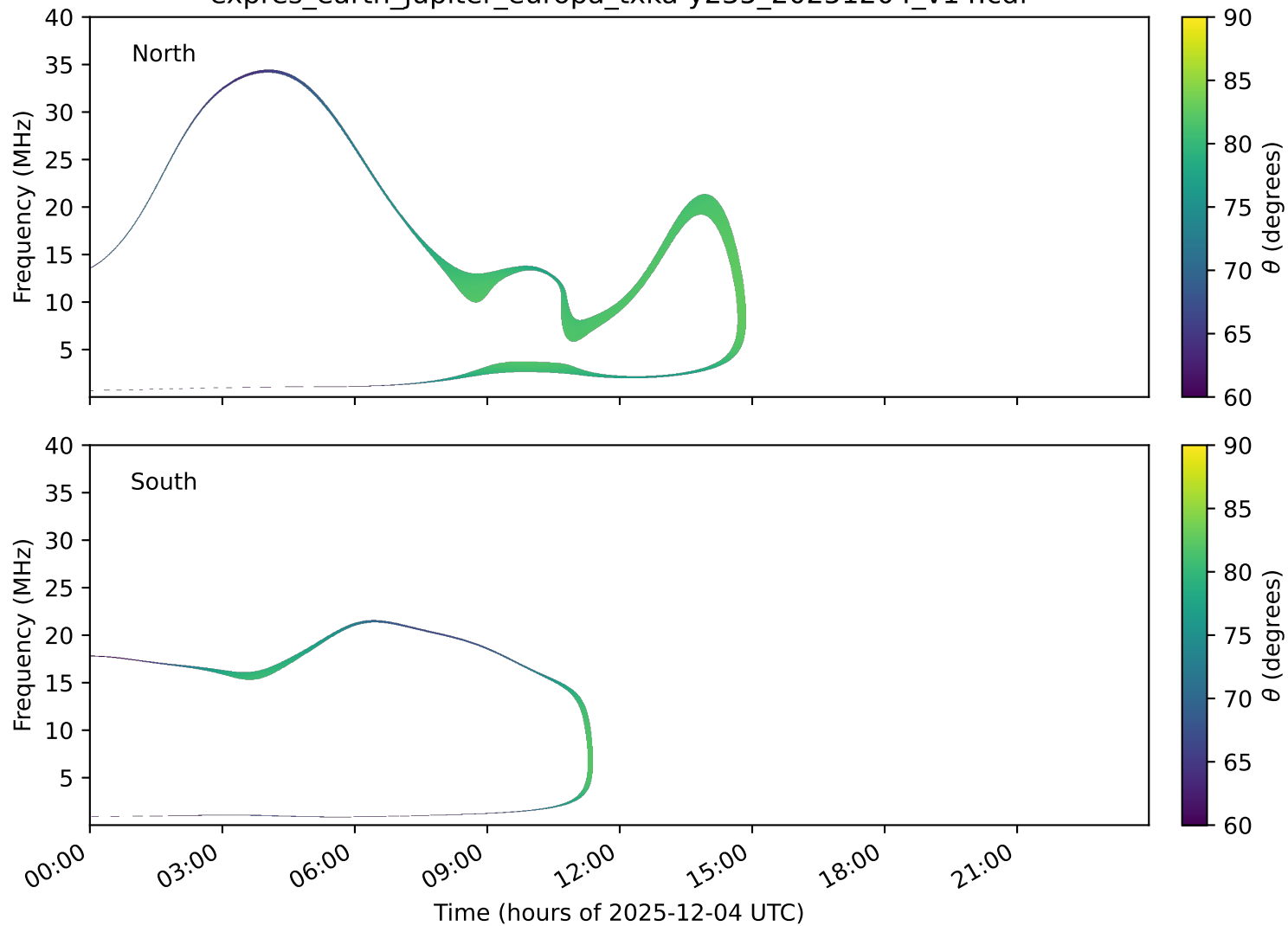
expres_earth_jupiter_europa_txka-y235_20251204_v14.cdf
