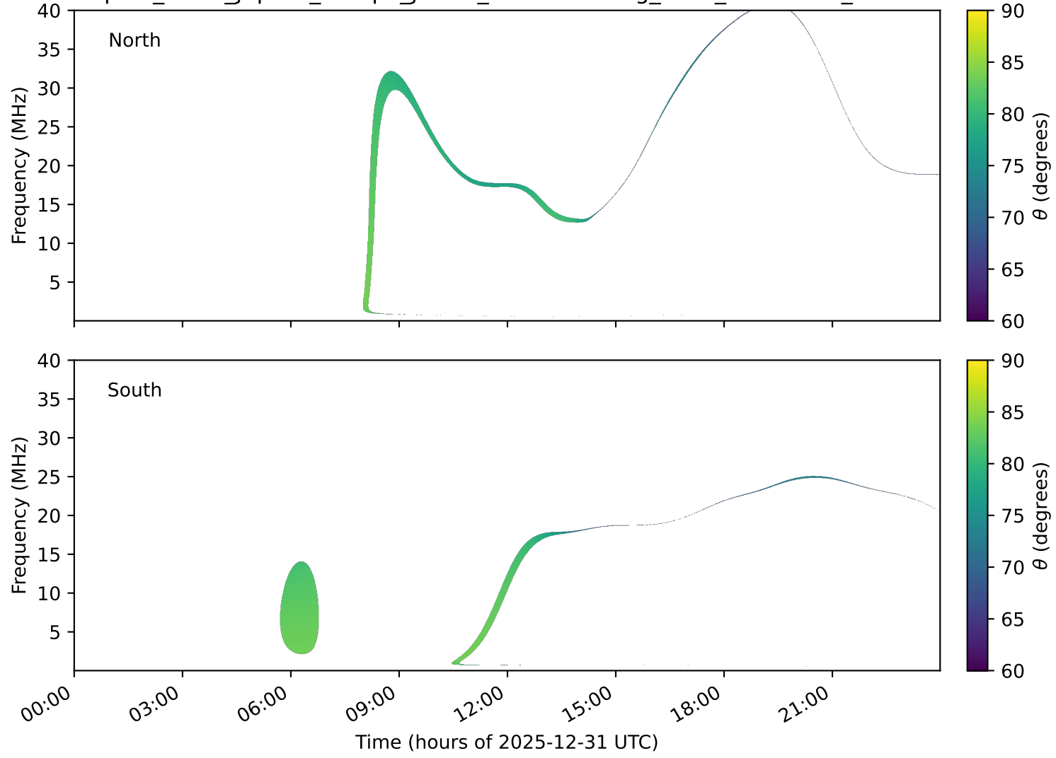
expres_earth_jupiter_europa_jrm33_lossc-wid1deg_3kev_20251231_v11.cdf
