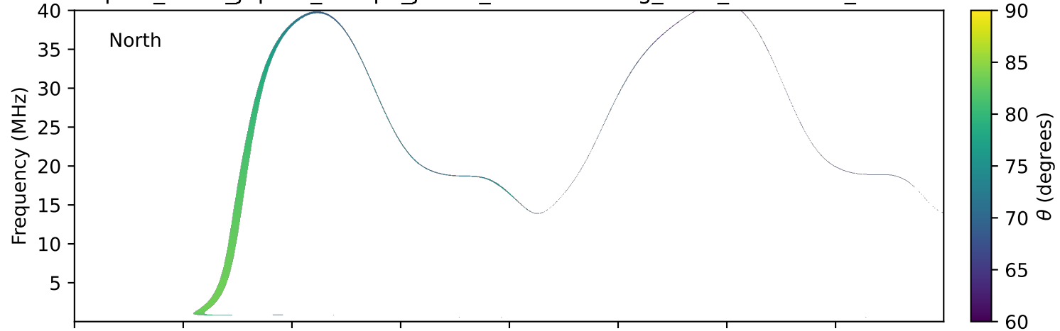
expres_earth_jupiter_europa_jrm33_lossc-wid1deg_3kev_20251210_v11.cdf
