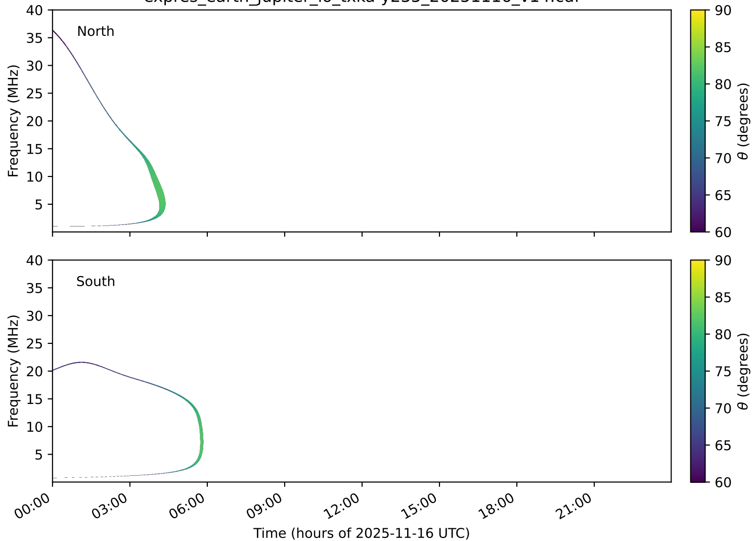
expres_earth_jupiter_io_txka-y235_20251116_v14.cdf
