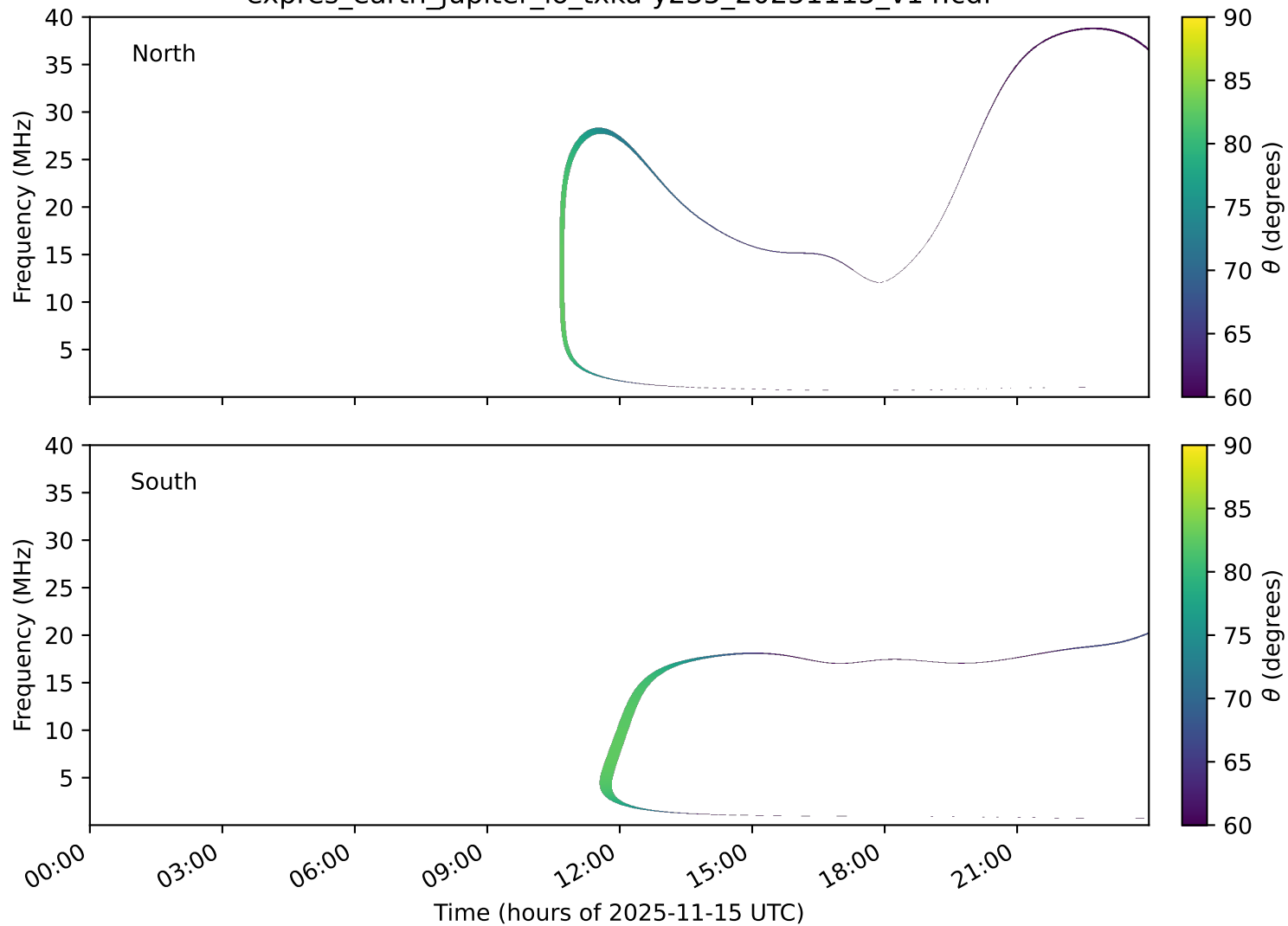
expres_earth_jupiter_io_txka-y235_20251115_v14.cdf
