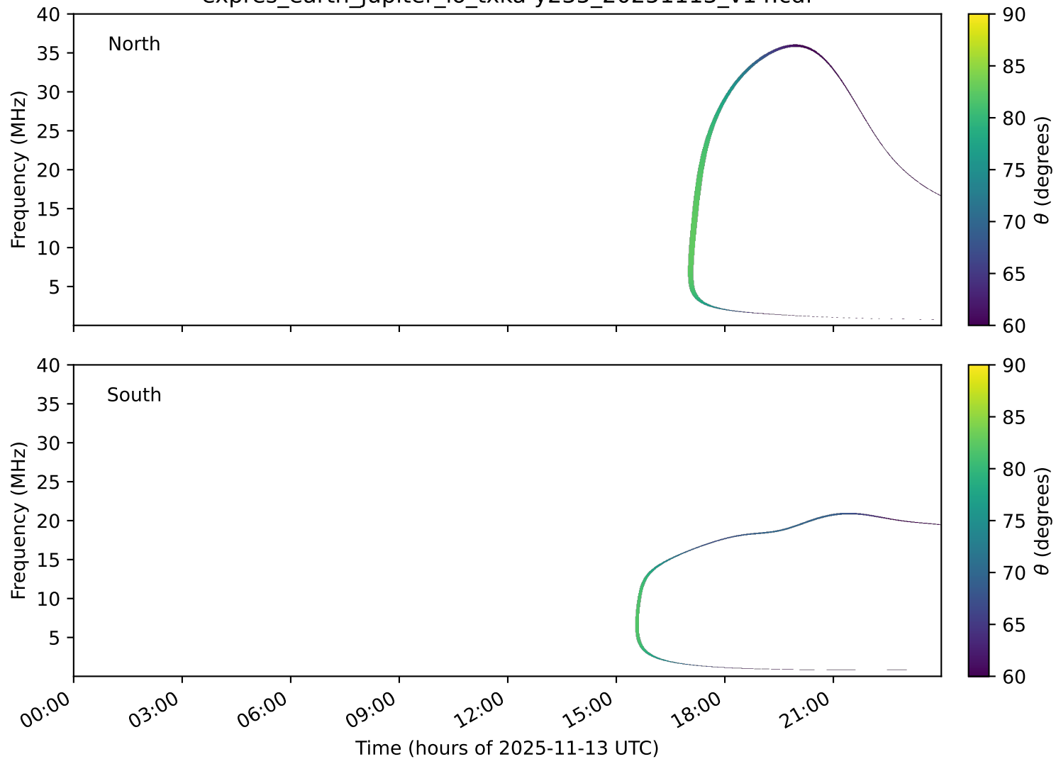
expres_earth_jupiter_io_txka-y235_20251113_v14.cdf
