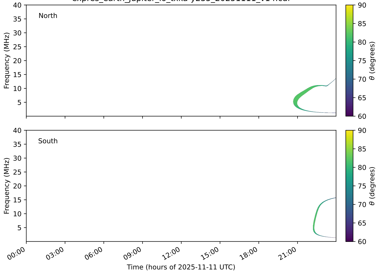
expres_earth_jupiter_io_txka-y235_20251111_v14.cdf
