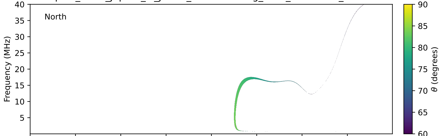
expres_earth_jupiter_io_jrm33_lossc-wid1deg_3kev_20251129_v11.cdf
