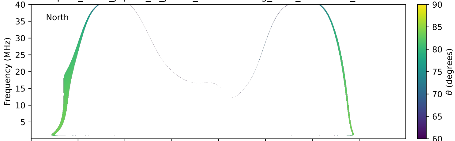
expres_earth_jupiter_io_jrm33_lossc-wid1deg_3kev_20251126_v11.cdf
