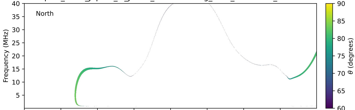
expres_earth_jupiter_io_jrm33_lossc-wid1deg_3kev_20251117_v11.cdf
