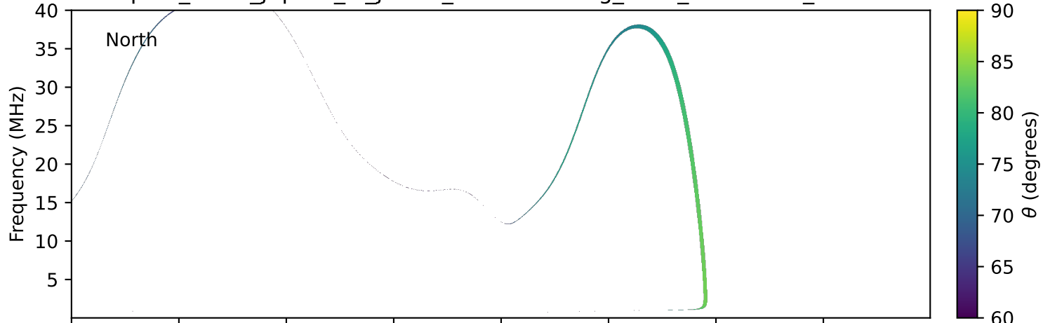
expres_earth_jupiter_io_jrm33_lossc-wid1deg_3kev_20251112_v11.cdf
