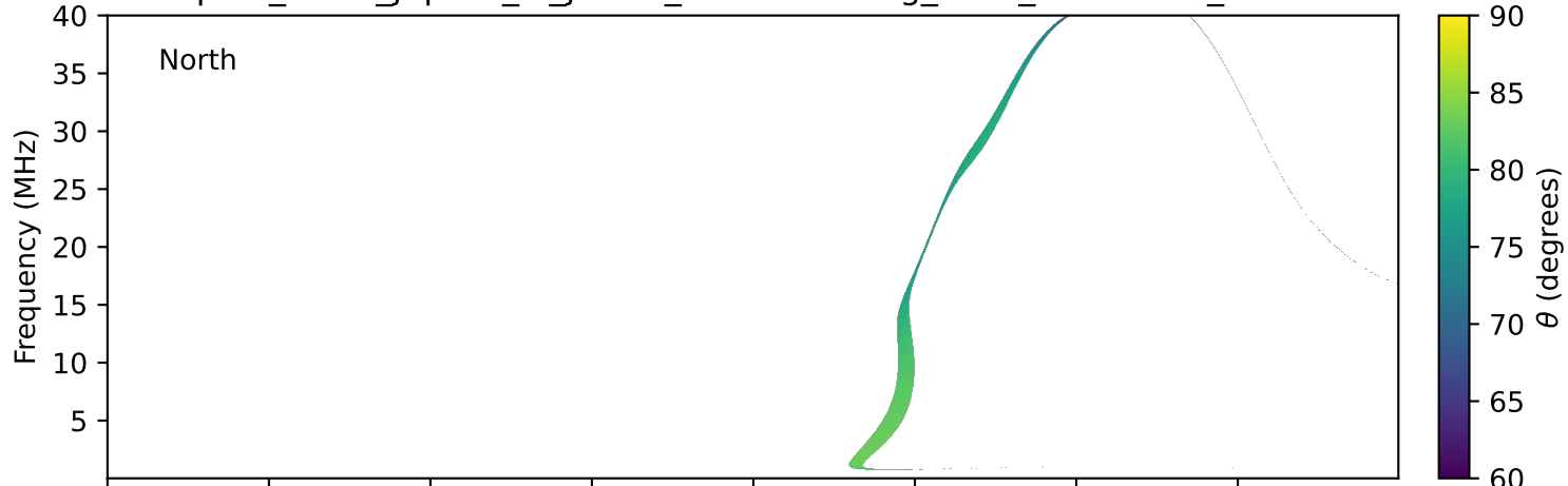
expres_earth_jupiter_io_jrm33_lossc-wid1deg_3kev_20251106_v11.cdf
