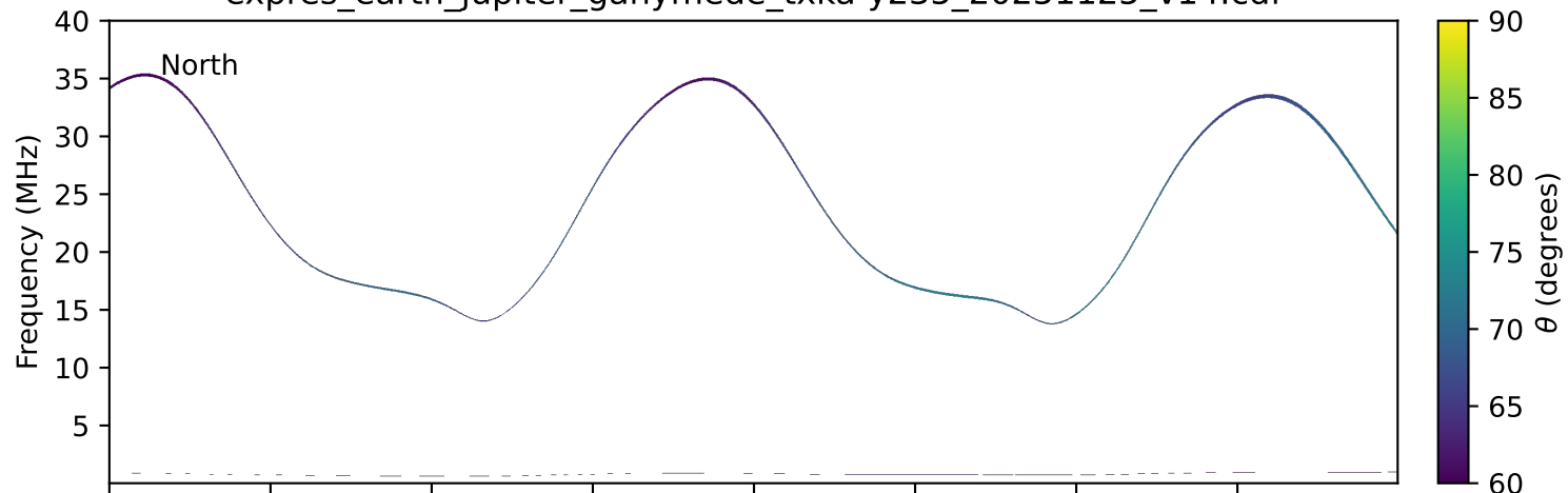
expres_earth_jupiter_ganymede_txka-y235_20251125_v14.cdf
