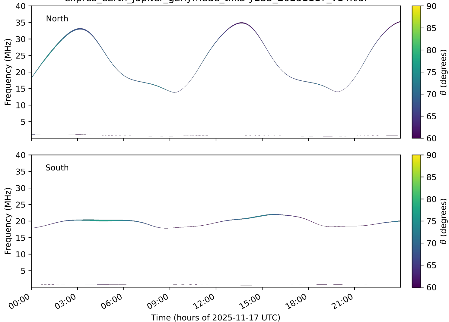
expres_earth_jupiter_ganymede_txka-y235_20251117_v14.cdf
