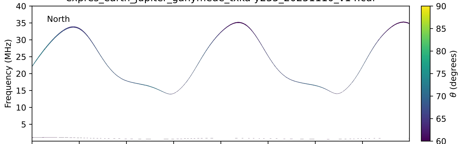
expres_earth_jupiter_ganymede_txka-y235_20251110_v14.cdf
