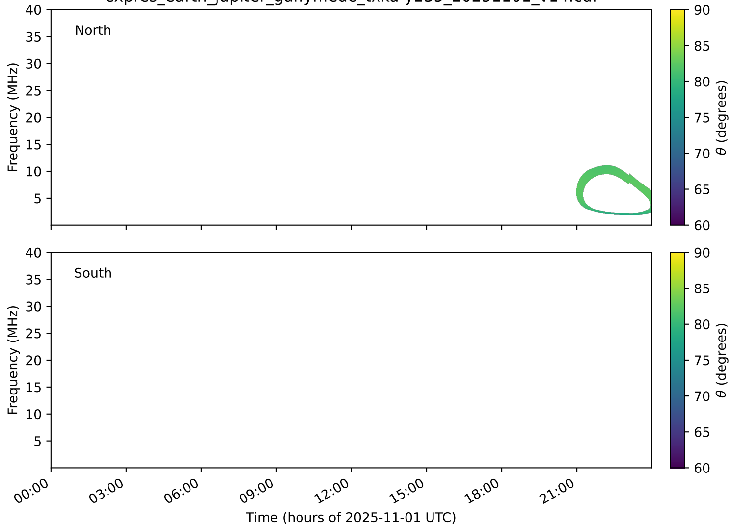
expres_earth_jupiter_ganymede_txka-y235_20251101_v14.cdf
